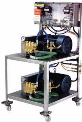
Modular System 1-2 bays, high pressure soap, rinse and wax
